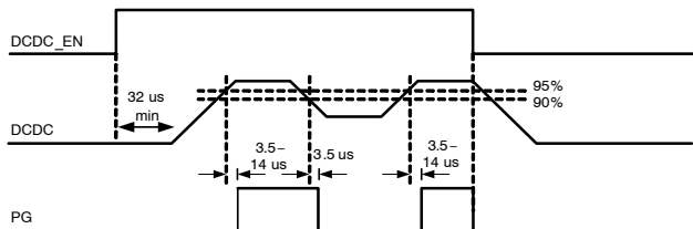
Figure 39. Power Good Signal
