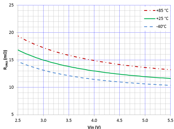
Figure 17. LSS R_{ON} vs. V_{IN} and Temperature
