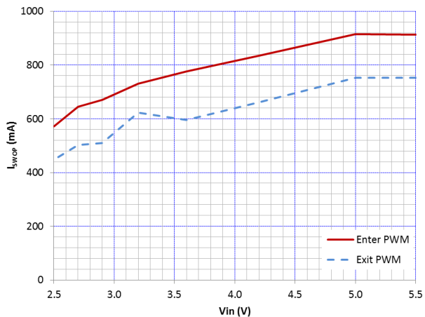
Figure 23. Switchover Point V_{OUT} = 1.4\text{ V}
