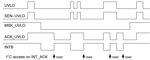
Figure 41. Interrupt Operation Example
