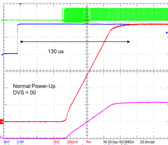
Figure 25. Normal Power Up, V_{OUT} = 1.15\text{ V} , DVS[1..0] = 00
