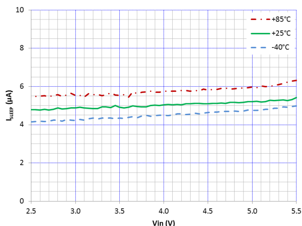
Figure 19. I_{SLEEP} vs. V_{IN} and Temperature
