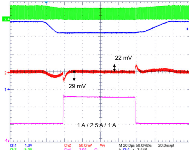
Figure 29. Transient Load 1 to 2.5 A Transient Line 3.9 to 3.3 V – Auto Mode
