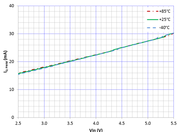
Figure 21. I_{Q\_PPWM} vs. V_{IN} and Temperature
