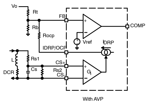
Figure 24. OCP Configuration
