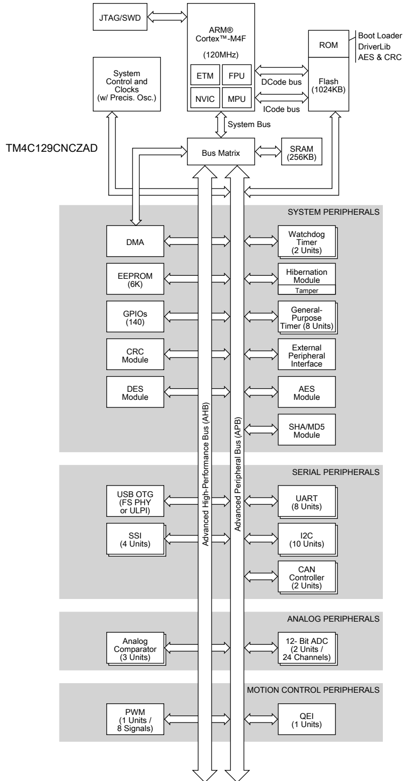
Figure 1-1. Tiva™ TM4C129CNCZAD Microcontroller High-Level Block Diagram
