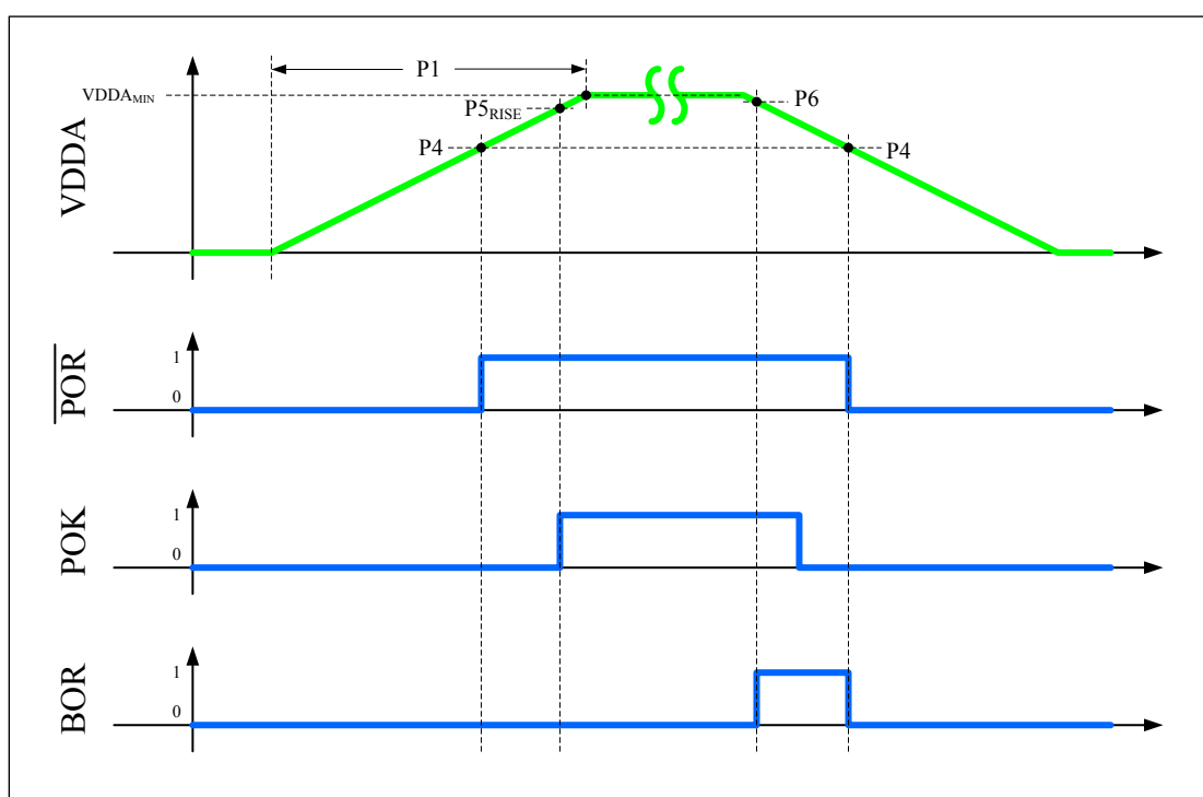
Figure 29-4. Power and Brown-Out Assertions vs V_{DDA} Levels
