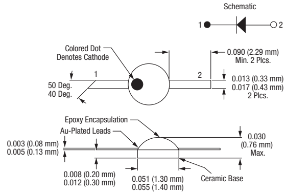
Figure 9. -230 Package Dimensions
