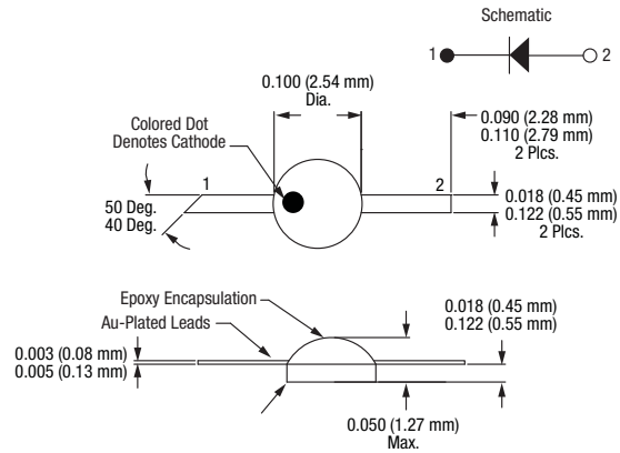
Figure 10. -250 Package Dimensions
