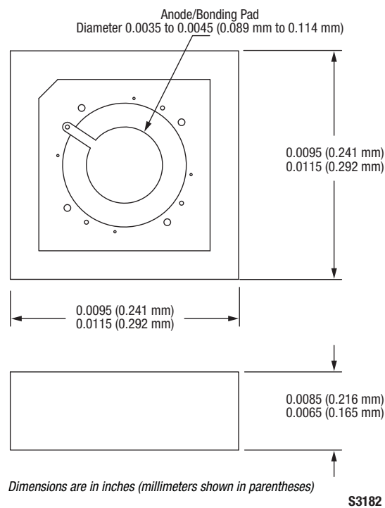
Figure 13. 571-011 Package Dimensions
