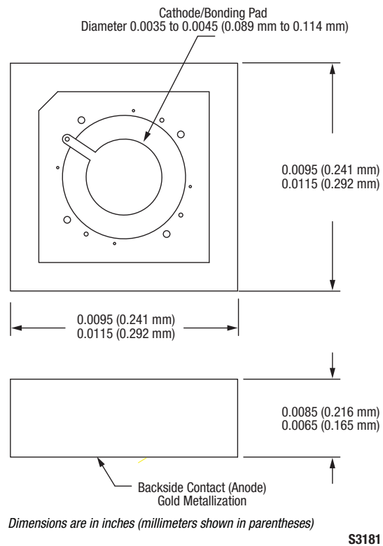
Figure 12. 571-006 Package Dimensions
