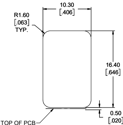
RECOMMENDED PANEL CUTOUT FOR EXTERNAL TABS PART NUMBER: NDM-X1XX1-00
