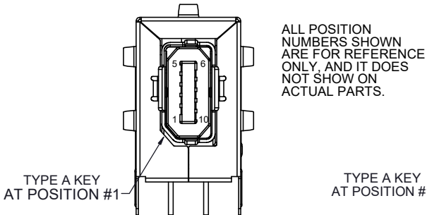
TYPE A KEY WITH EXTERNAL TABS PART NUMBER: NDM-A1XX1-00
