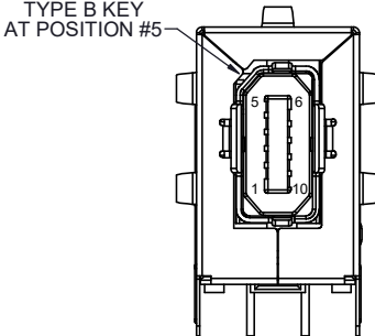
TYPE B KEY WITH EXTERNAL TABS PART NUMBER: NDM-B1XX1-00
