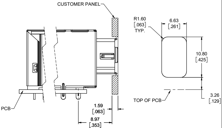
RECOMMENDED PANEL CUTOUT WITHOUT EXTERNAL TABS PART NUMBER: NDM-X2XX1-00
