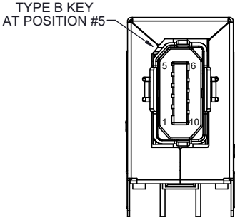
TYPE B KEY WITHOUT EXTERNAL TABS PART NUMBER: NDM-B2XX1-00
