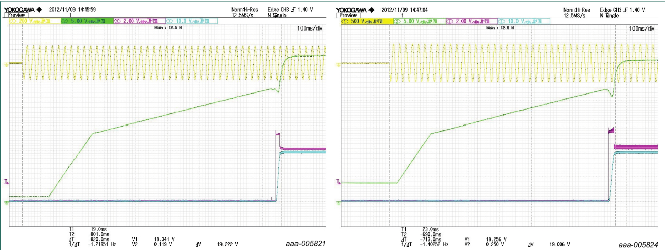
a. Mains input 90 V/60 Hz; delay time: 820 ms b. Mains input 264 V/50 Hz; delay time: 713 ms (1) Load = 4.62 A (2) Ch1 (yellow): mains input (3) Ch2 (green): VCC pin TEA1755 (4) Ch3 (magenta): FBCTRL pin TEA1755 (5) Ch4 (cyan): output voltage
