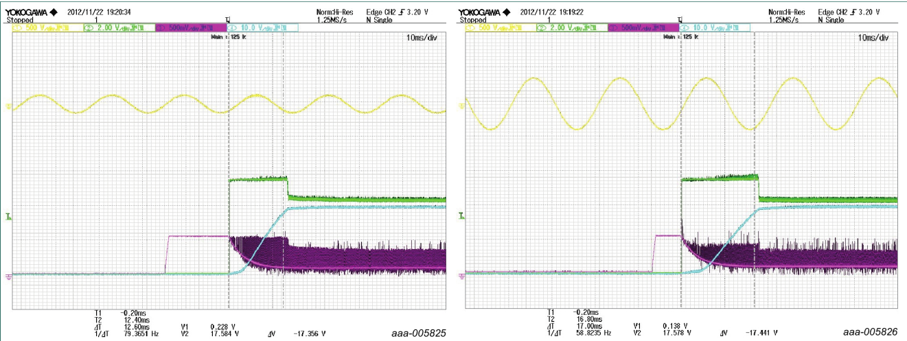
a. Mains input 90 V/60 Hz; output rise time: 13 ms b. Mains input 264 V/50 Hz; output rise time: 17 ms (1) Load = 4.62 A (2) Ch1 (yellow): mains input (3) Ch2 (green): FBCTRL pin TEA1755 (4) Ch3 (magenta): FBSENSE pin TEA1755 (5) Ch4 (cyan): output voltage
