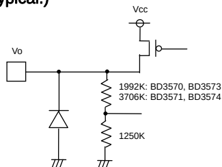
Fig.17 5PIN[Vo] BD3570,3571,3573,3574
