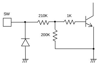
Fig.16 2PIN[SW]
