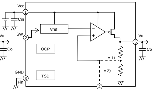
Fig.15 HRP5
