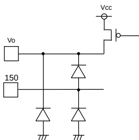
Fig.18 4.5PIN[ADJ,Vo] BD3572,BD3575
