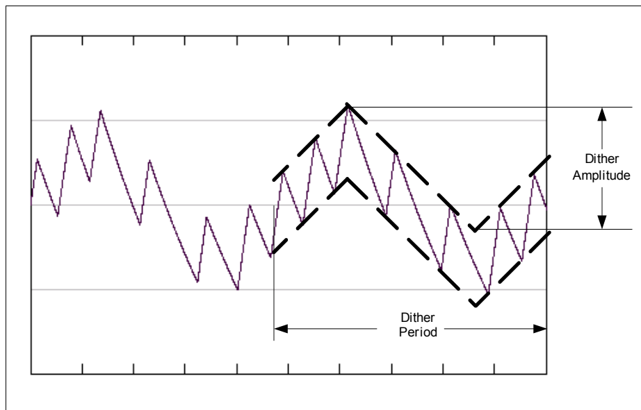
Figure 18 Dither Waveform
