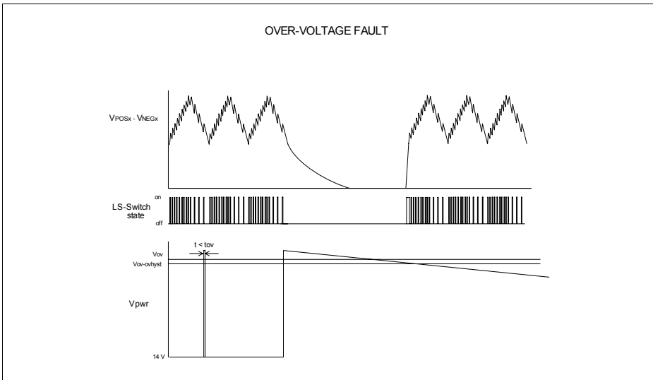
Figure 4 Overvoltage Shutdown
