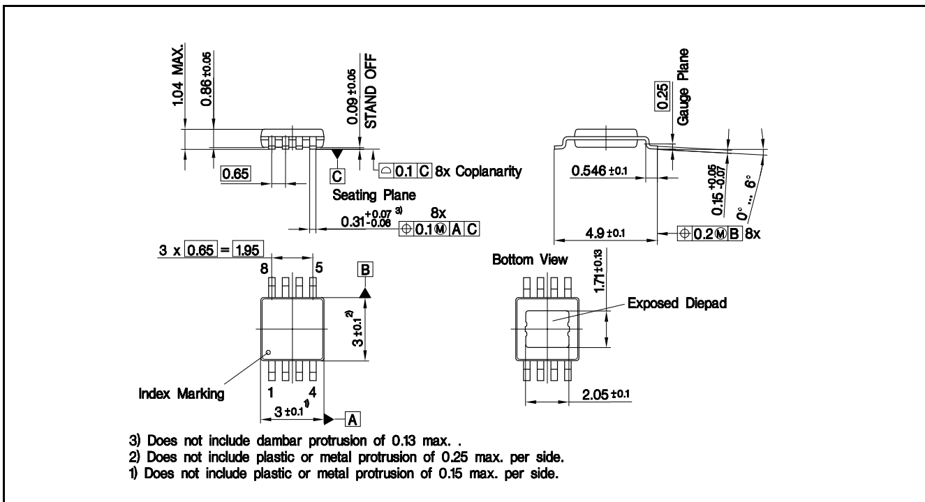
Figure 22 PG-TSSOP-8-1 outline
