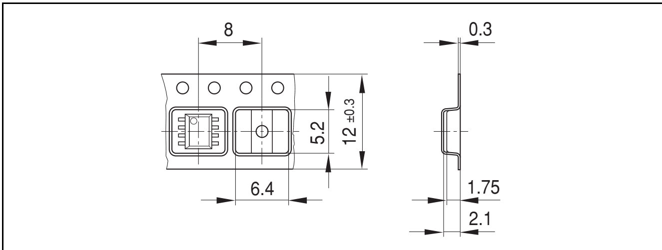
Figure 21 PG-DSO-8-60 packaging
