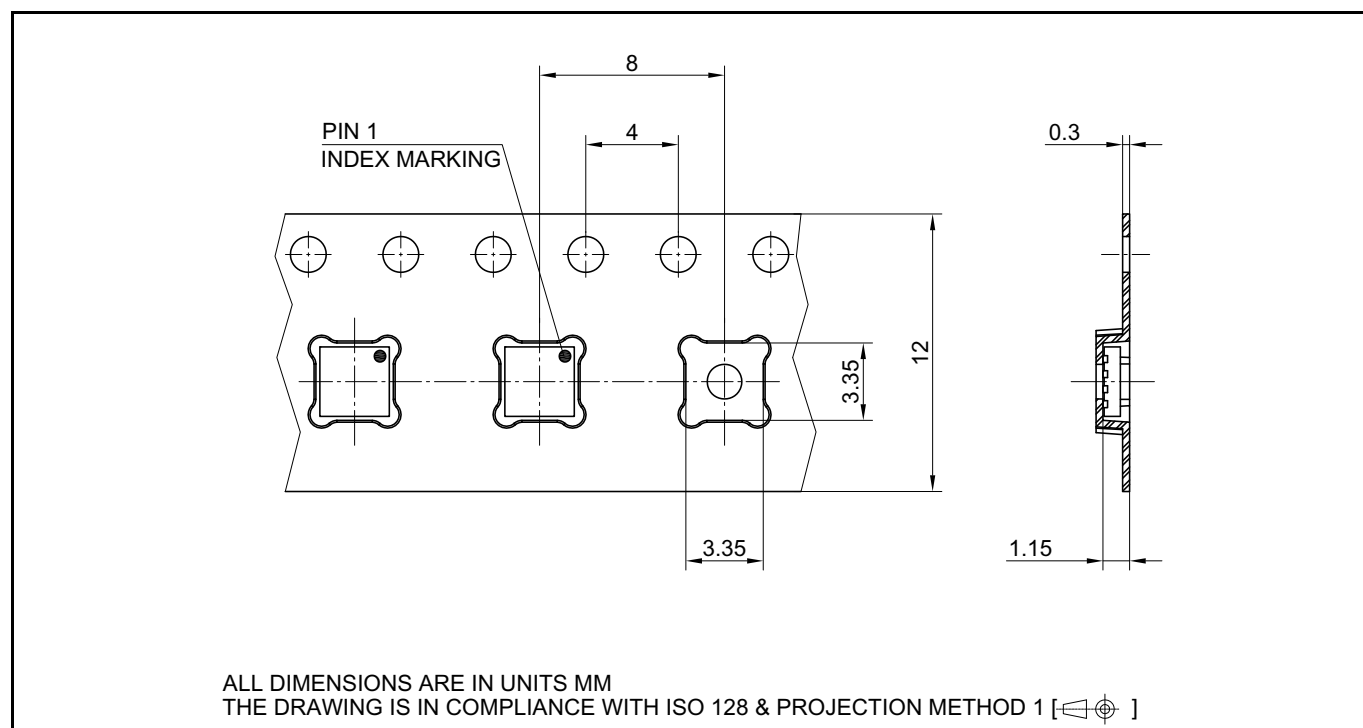
Figure 27 PG-WSO8-3 packaging
