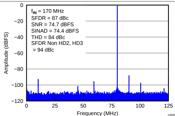
Figure 6. FFT for 170-MHz Input Signal ( 2.5\text{-V}_{PP} Full-Scale)
