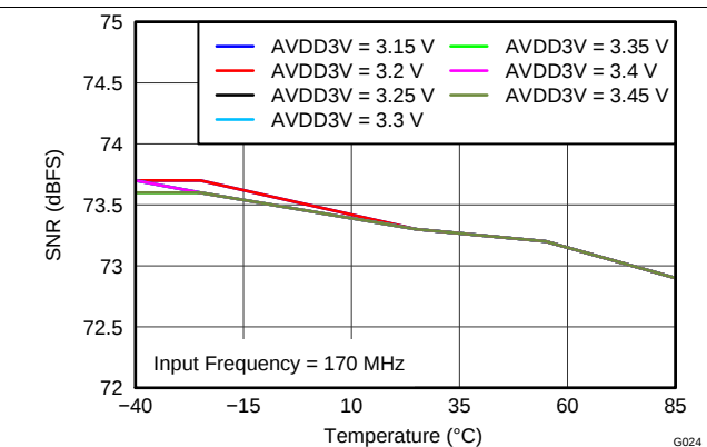
Figure 23. Signal-to-Noise Ratio vs AVDD Supply and Temperature (170 MHz)
