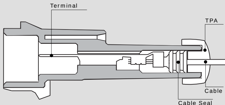
Male Connector
