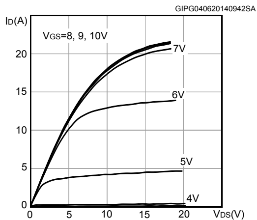
Figure 3. Output characteristics
