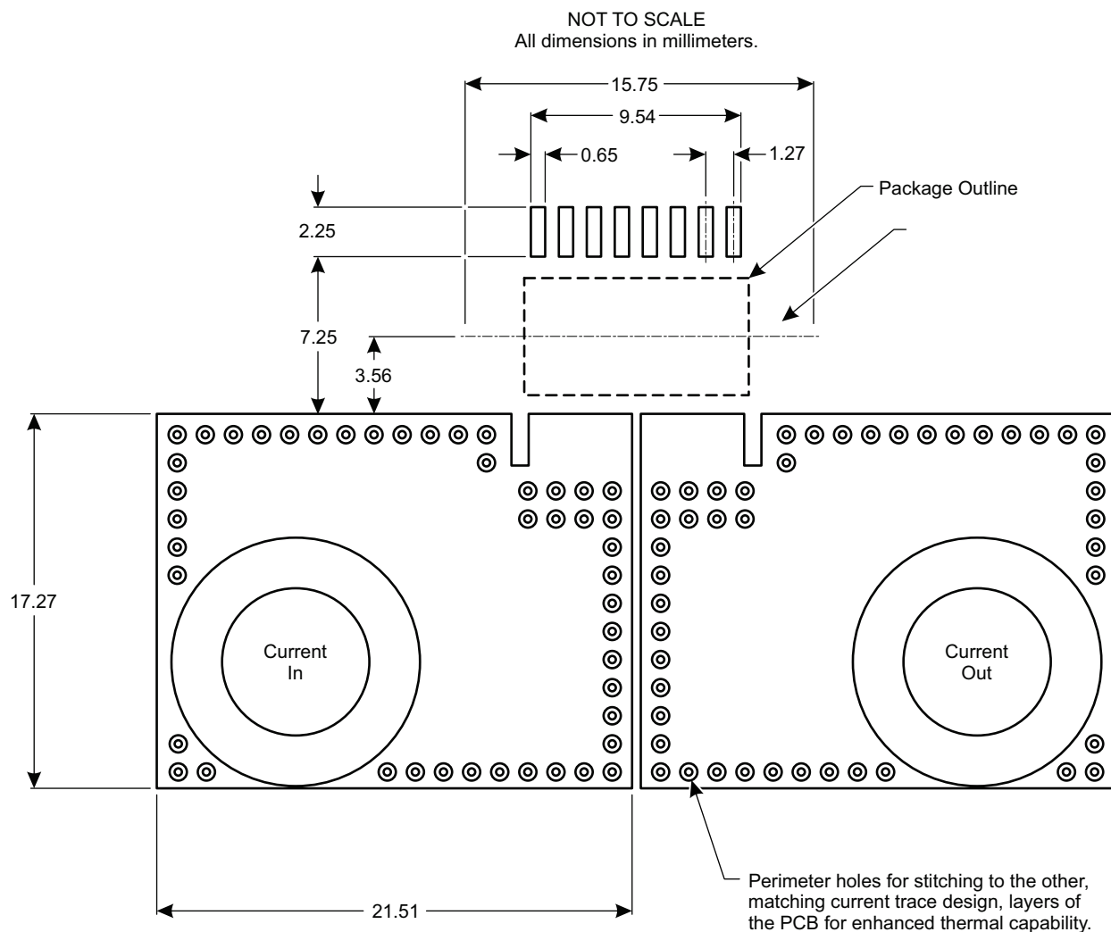
Figure 17: High Isolation PCB Layout
