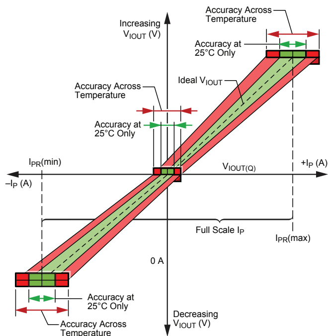
Figure 12: Output Voltage versus Sensed Current
