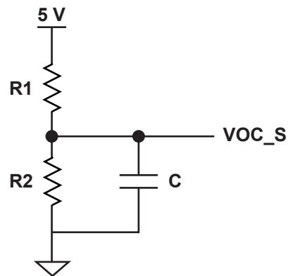
Figure 4: Resistor Divider
