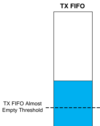
Figure 12. TX FIFO
