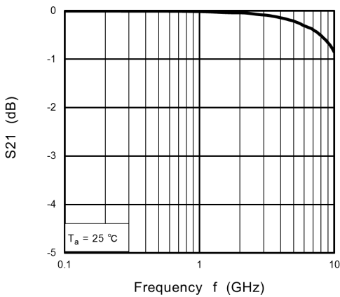
Fig. 9.5 S_{21} - f
