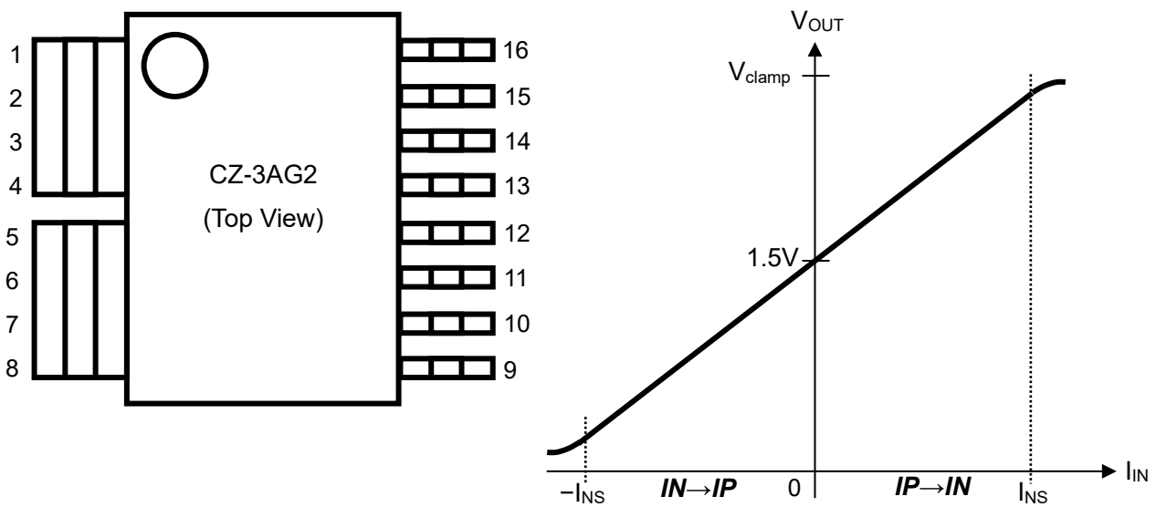
Figure 2. Pin configurations and typical output characteristics of CZ-3AG2
