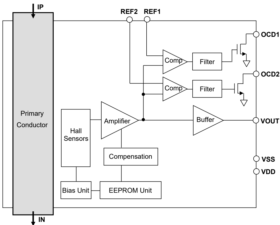
Figure 1. Block diagram of CZ-3AG2
