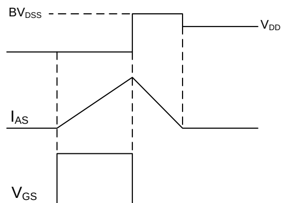
Figure 12. EAS Waveform
