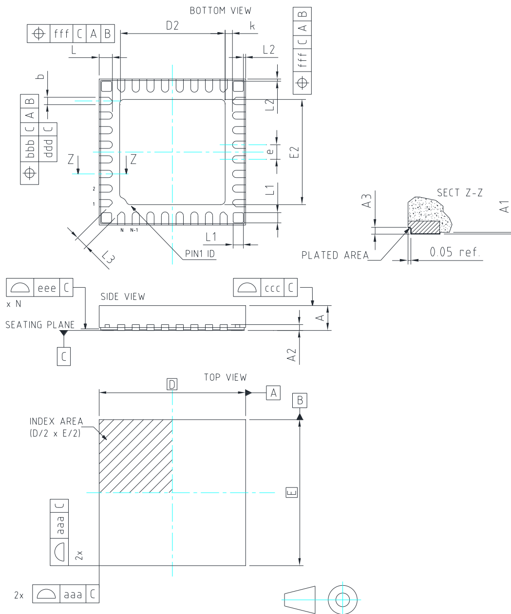
Figure 20. VFQFN (5x5x0.9, 32+4L) package outline
