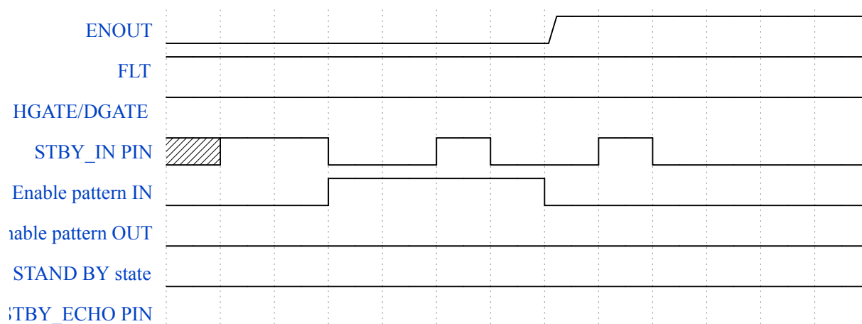
Figure 16. Standby pattern during ENOUT low state
