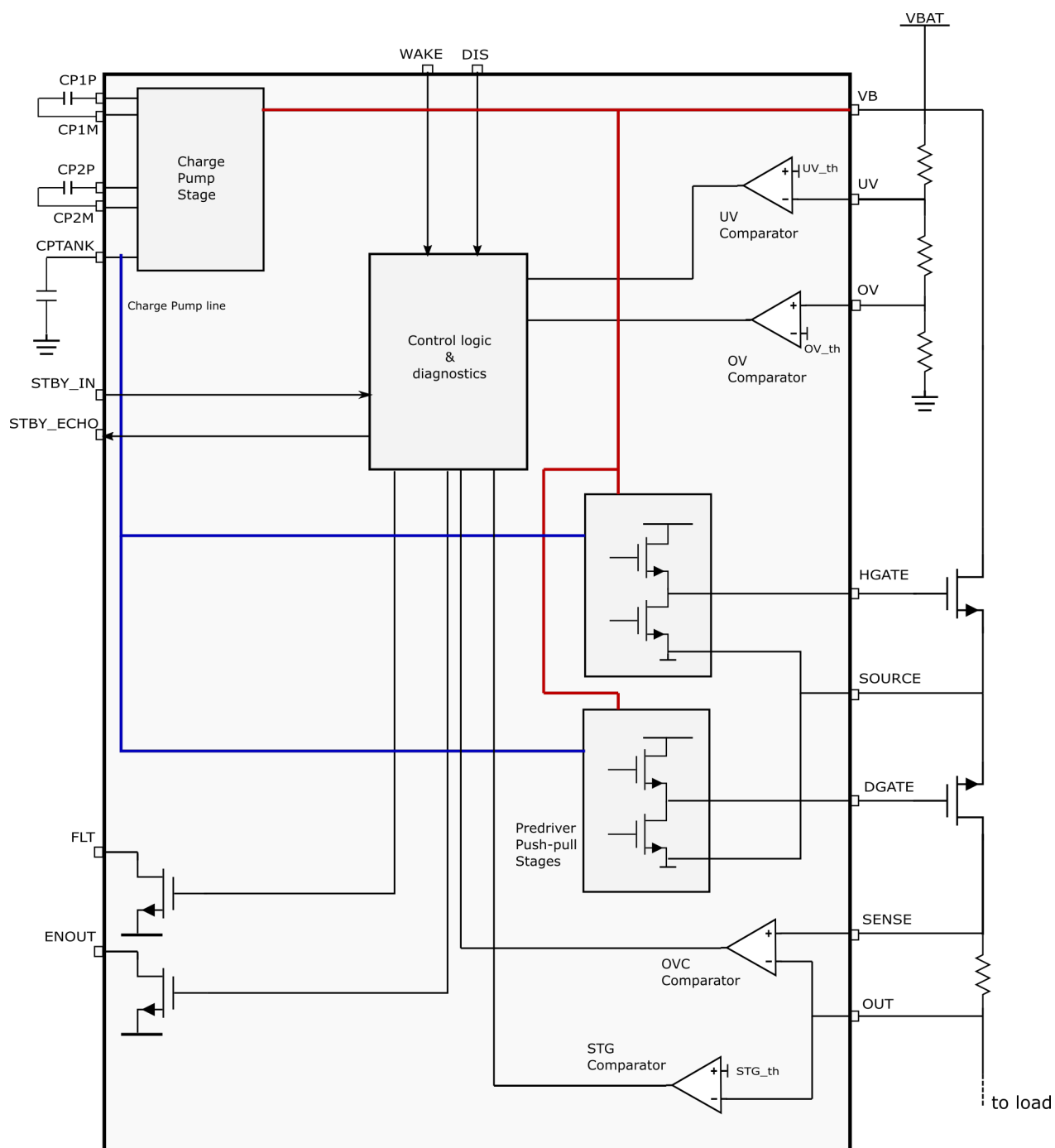
Figure 1. STPM801 Block diagram
