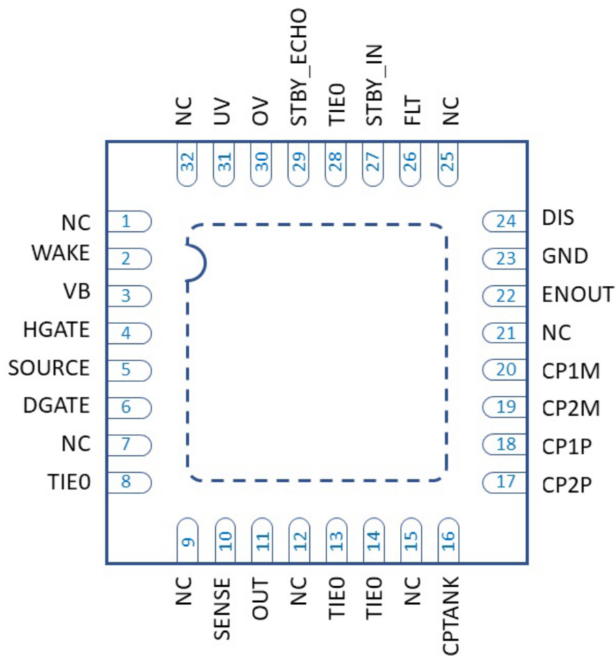
Figure 2. Pin out (top view)
