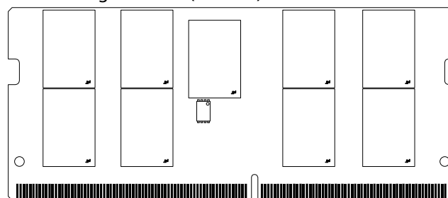
Figure 2: 260-Pin SODIMM (R/C G1)
