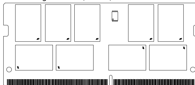
Figure 2: 260-Pin SODIMM (R/C G1)
