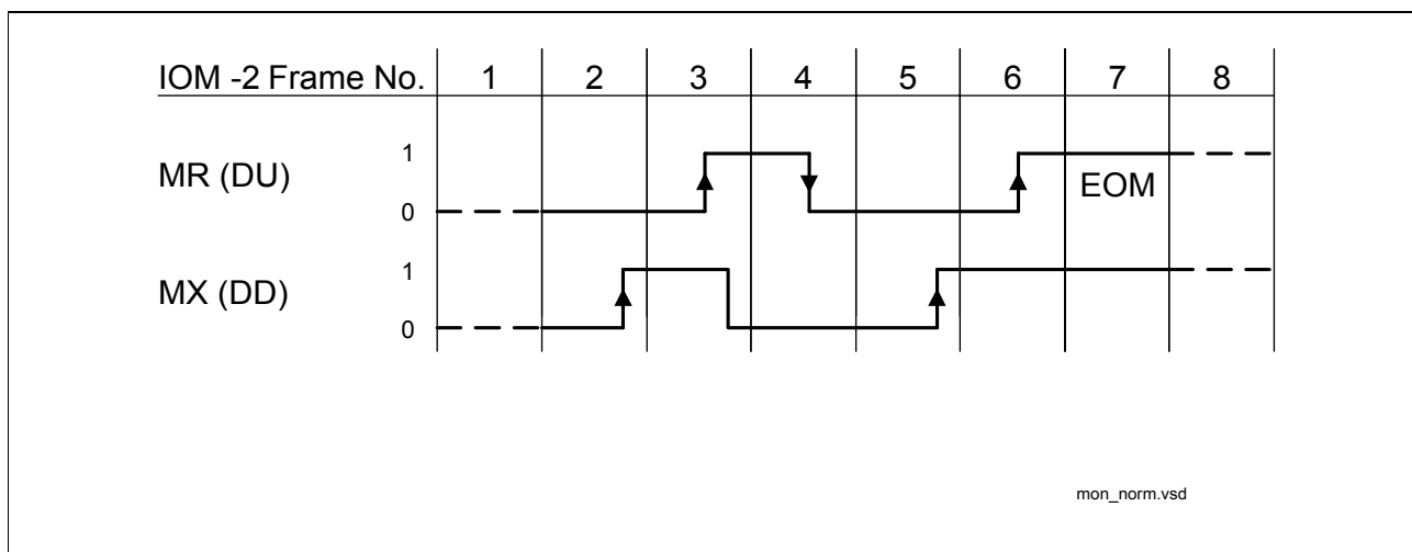
Figure 69 Monitor Channel, Normal End of Transmission
