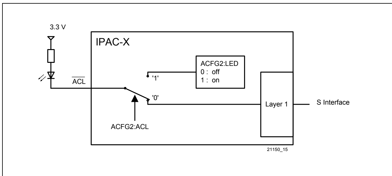
Figure 17 ACL Configuration
