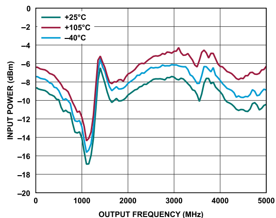
Figure 26. Minimum Input Signal for REF_OK = 1 for Delayed Match Amplifier (DMA) Buffer at Various Temperatures
