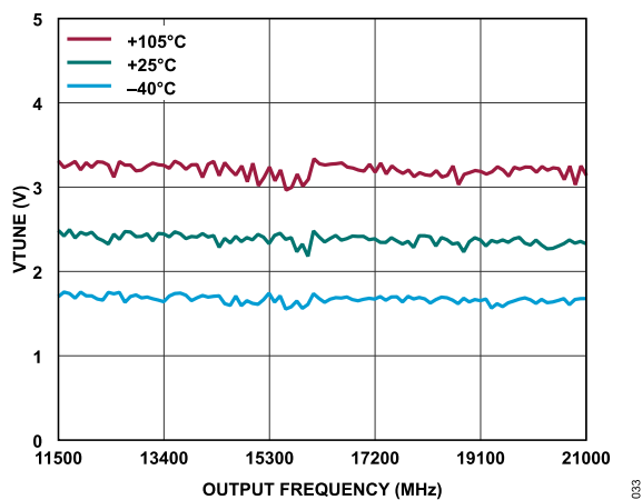
Figure 33. VTUNE vs. Output Frequency at Various Temperatures
