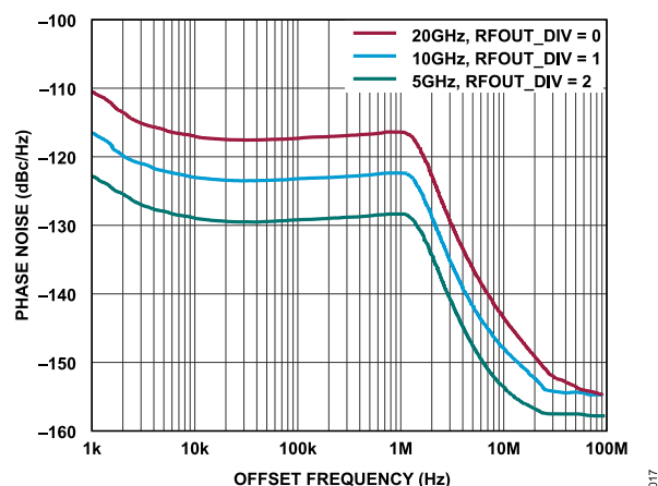
Figure 17. Closed-Loop Phase Noise vs. Offset Frequency at 20 GHz VCO Frequency and Divided Output Frequency
