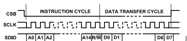
Figure 50. Serial Interface, LSB First (LSB_FIRST = 1)
