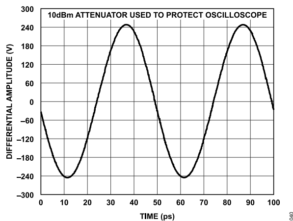
Figure 40. Differential Amplitude vs. Time at 20 GHz
