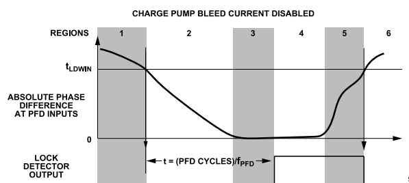
Figure 45. Lock Detector Timing, Bleed Current Disabled
