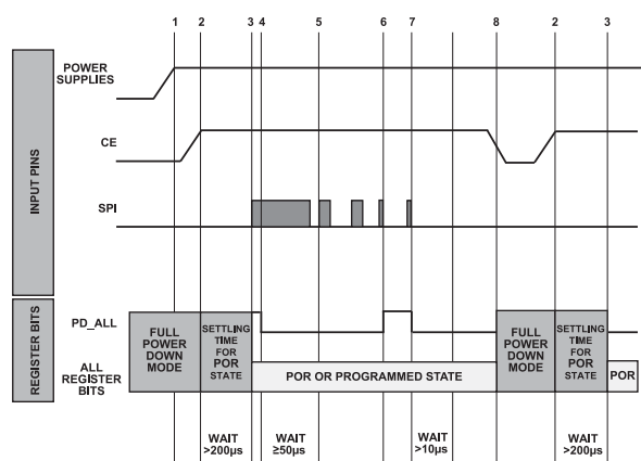
Figure 56. Power-Up and Initialization
