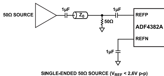
Figure 57. Single-Ended 50 \Omega Source ( V_{REF} < 2.6 \text{ V p-p} )
