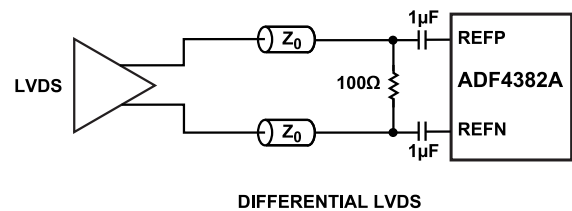
Figure 61. Differential LVDS
