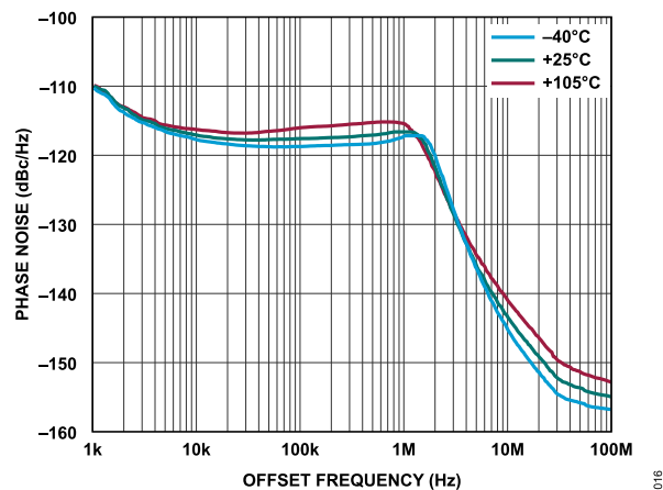
Figure 16. Closed-Loop Phase Noise vs. Offset Frequency at 20 GHz VCO Frequency Across Temperatures
