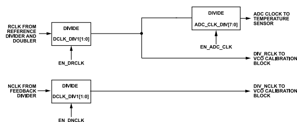
Figure 52. VCO Calibration Dividers
