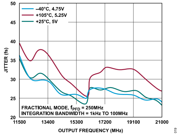
Figure 19. 1 kHz to 100 MHz Integrated Jitter in Fractional Mode, f_{PFD} = 250 MHz
