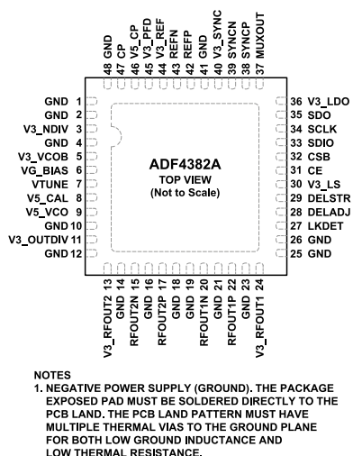
Figure 6. Pin Configuration
