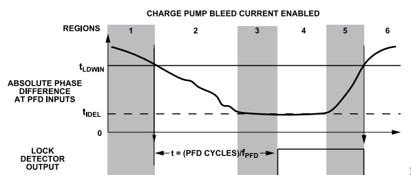
Figure 46. Lock Detector Timing, Bleed Current Enabled
