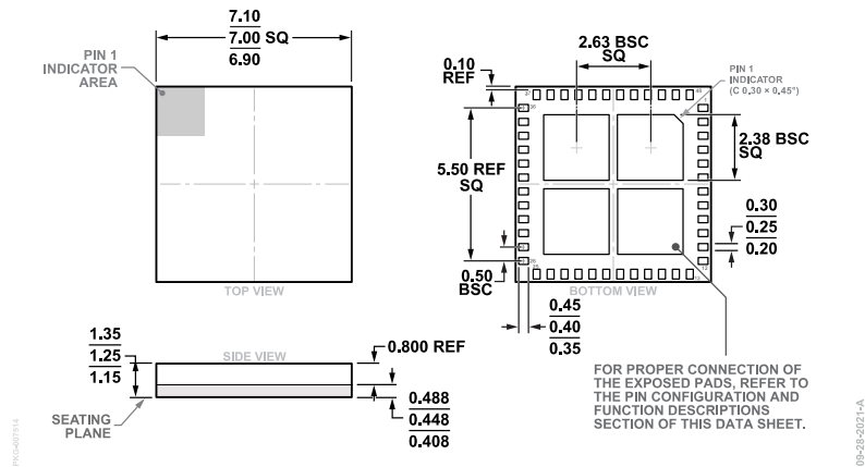
Figure 66. 48-Terminal Land Grid Array Package [LGA] (CC-48-10) Dimensions shown in millimeters
