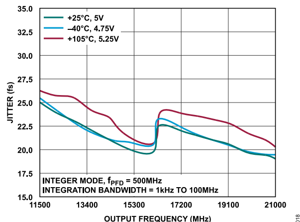
Figure 18. 1 kHz to 100 MHz Integrated Jitter in Integer Mode, f_{PFD} = 500 MHz
