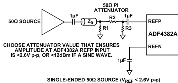
Figure 58. Single-Ended 50 \Omega Source ( V_{REF} < 2.6 \text{ V p-p} )
