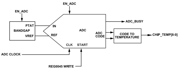
Figure 48. Temperature Sensor
