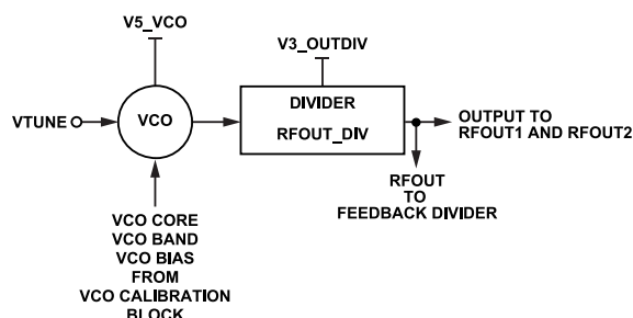
Figure 51. VCO and Clock Output Divider
