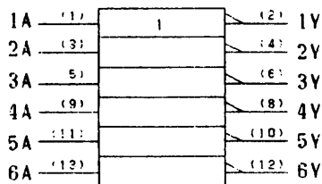
LOGIC SYMBOL
