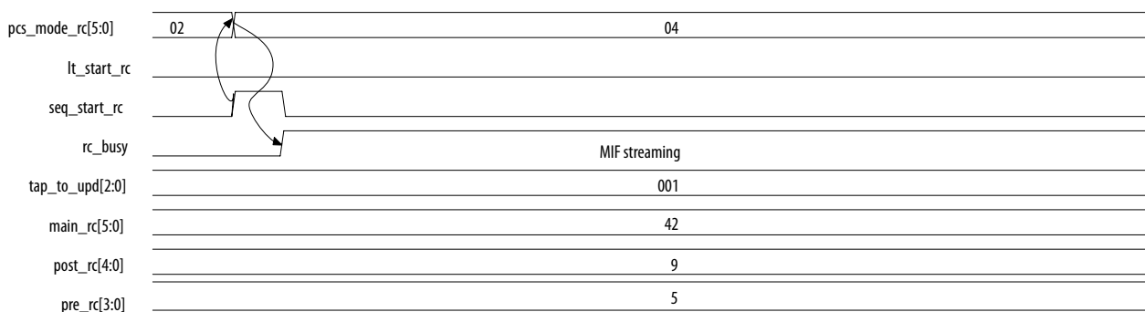
Figure 4-6: Transition from Link Training to Data Mode
