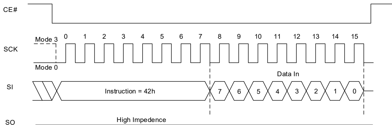
Figure 8.51 Write Function Register Sequence In SPI Mode
