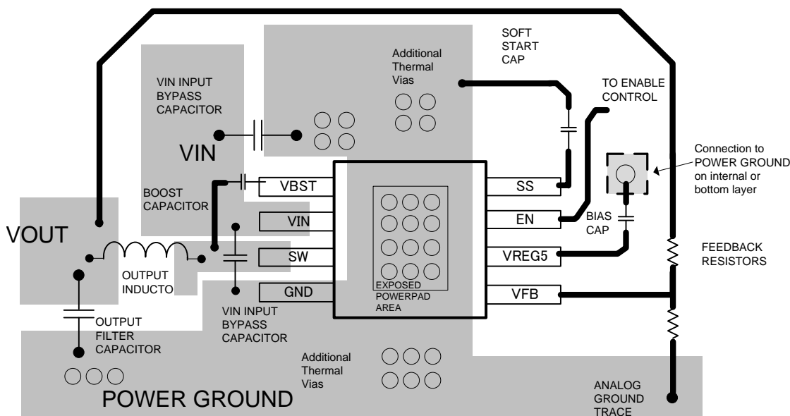
Figure 16. PCB Layout
