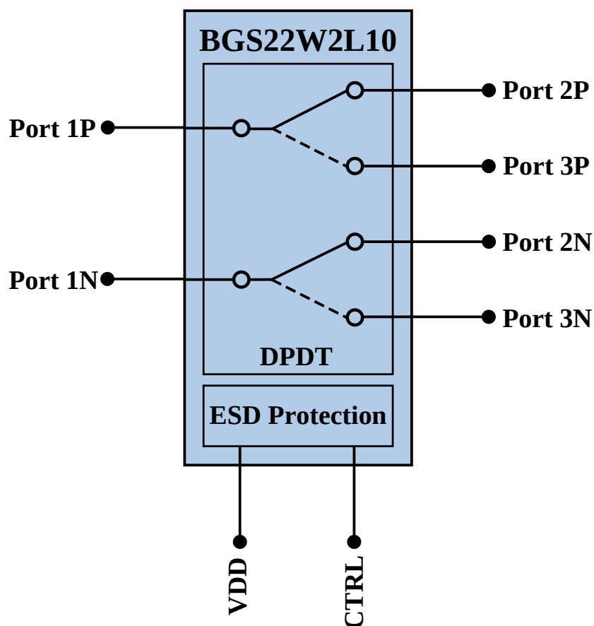
Figure 1: BGS22W2L10 Block Diagram
