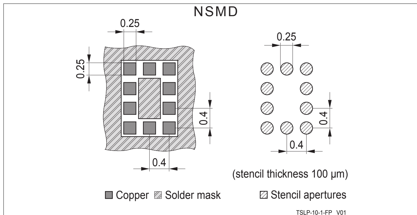
Figure 4: Footprint TSLP-10-1
