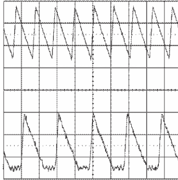
Figure 35. CCM and DCM Operating Modes V_{IN} = 12 \text{ V} , V_O = 3.3 \text{ V} , I_O = 1 \text{ A} / 0.25 \text{ A}
