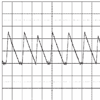
Figure 36. Transition Mode Operation V_{IN} = 24 \text{ V} , V_O = 3.3 \text{ V} , I_O = 0.29 \text{ A}
