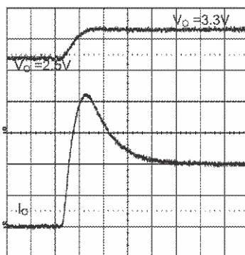
Figure 33. Prebiased Start-Up
