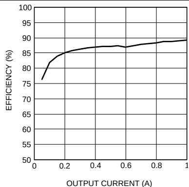
Figure 37. Efficiency V_{IN} = 24\text{ V} V_{OUT} = 5\text{ V}
