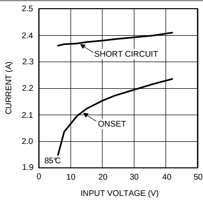
Figure 31. Current Limit 3.3 V_{OUT} at 85^\circ\text{C}
