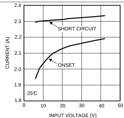
Figure 30. Current Limit 3.3\text{ V}_{OUT} at 25^\circ\text{C}
