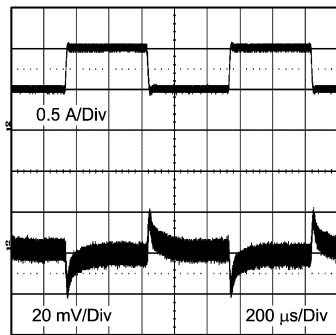
Figure 25. Line and Load Regulation at -55^\circ\text{C}
