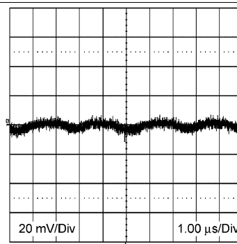
Figure 26. Output Ripple 24\text{-}V_{IN} 3.3\text{-}V_O 1\text{-A} , BW = 200\text{ MHz}
