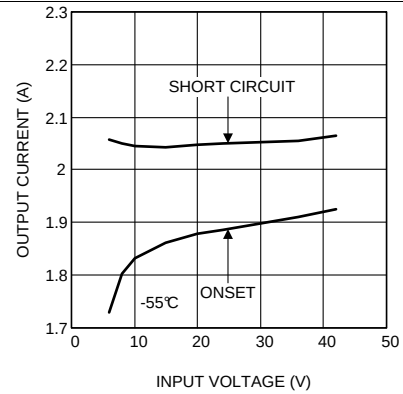
Figure 32. Current Limit 3.3 V_{OUT} at -55^\circ\text{C}
