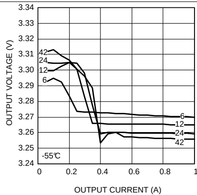
Figure 25. Line and Load Regulation at -55^\circ\text{C}
