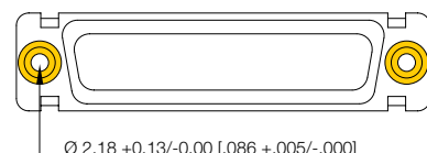
\varnothing 2.18 + 0.13 / - 0.00 [.086 + .005 / - .000] clearance holes, two places
