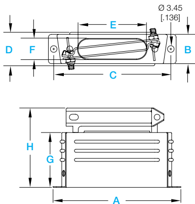
H Backshell, metal, top entry
