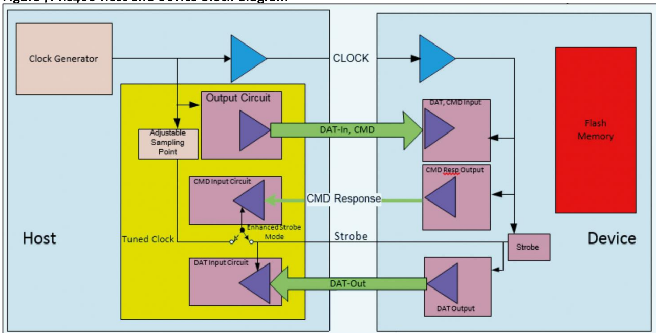
Figure 7: HS400 Host and Device block diagram
