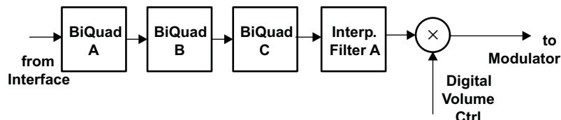
Figure 5-19. Signal Chain for PRB_P1 and PRB_P4
