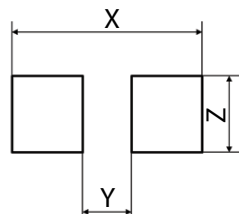
SUGGESTED LAND PATTERN
