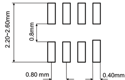
SUGGESTED LAND PATTERN
