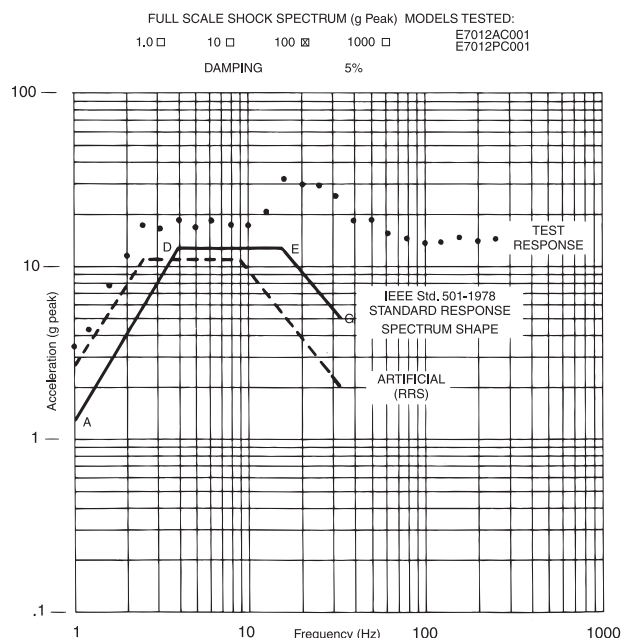
Figure 1. Response Spectrum, Transitional Mode
