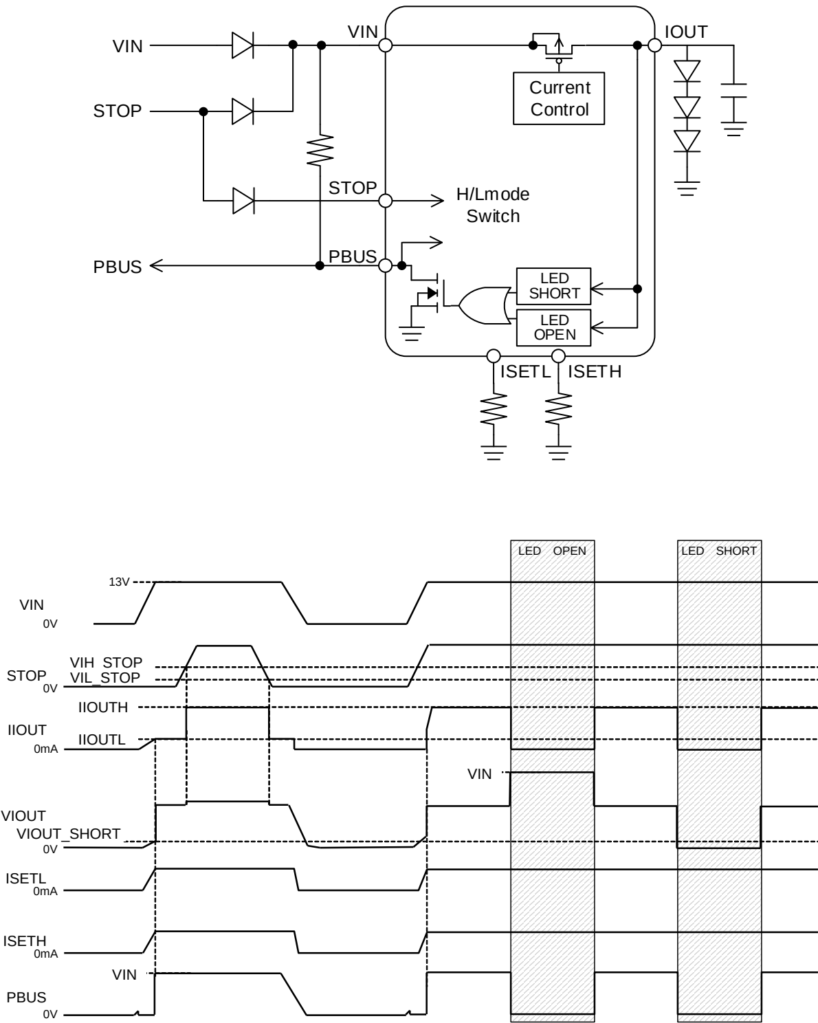
Figure 13. Timing Chart
