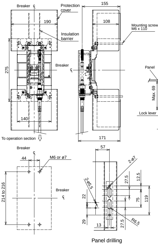
Drive section
