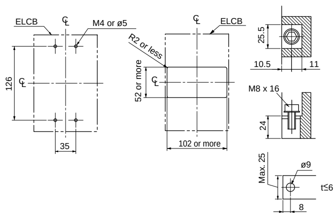
Panel drilling
