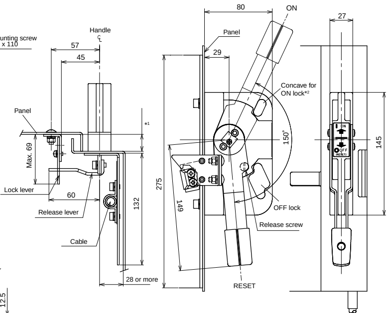
Operation section
