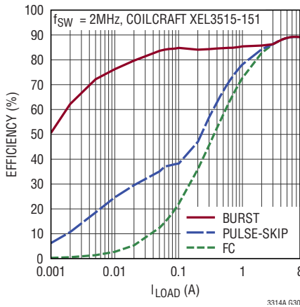
2-Phase Efficiency vs Load, 5.0V to 1.0V
