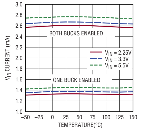
PV_{\text{IN}} Quiescent Current, All Modes, Not Sleeping
