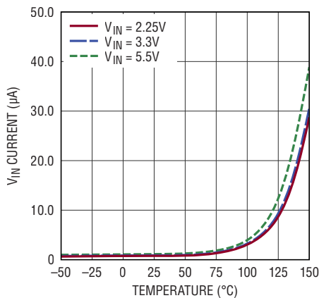
PV_{\text{IN}} Shutdown Current
