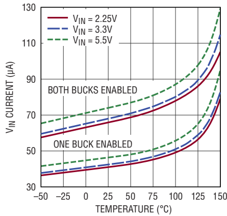
PV_{\text{IN}} Quiescent Current, Burst Mode Operation, Sleeping
