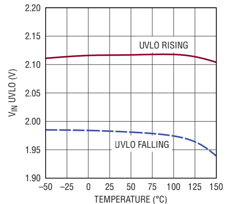
PV_{\text{IN}} UVLO Threshold
