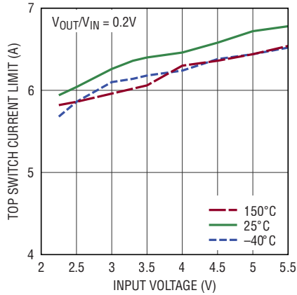
Top Switch Current Limit vs V_{\text{IN}}
