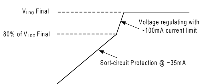
Figure 8 — LDO Start-Up
