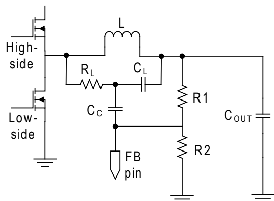
Figure 10 — Signal Injection Circuit
