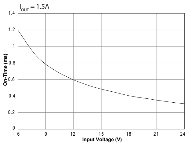
On-Time vs. V_{IN}
