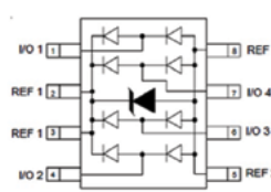
Pin configuration
