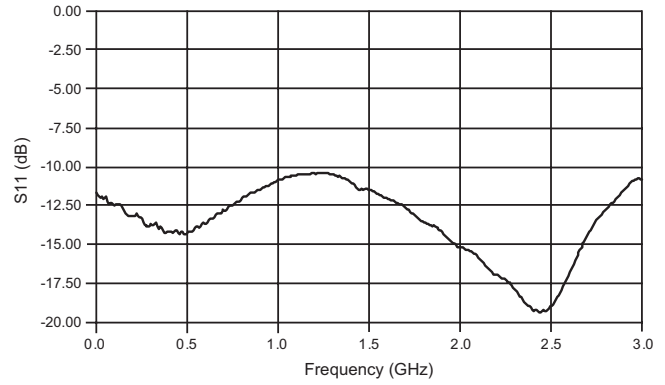
Typical Return Loss Curve, S11
