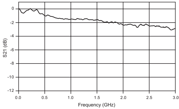
Typical Frequency Response Curve, S21
