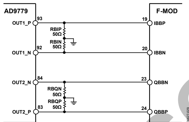
Figure 29. Interface Between the AD9779 and ADL5374 with 50 \Omega Resistors to Ground to Establish the 500 mV dc Bias for the ADL5374 Baseband Inputs
