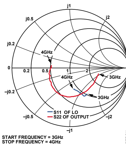
Figure 8. Smith Chart of LOIP (LOIN AC-Coupled to Ground) S11 and VOUT S22 ( f_{\text{LO}} from 3000 MHz to 4000 MHz)
