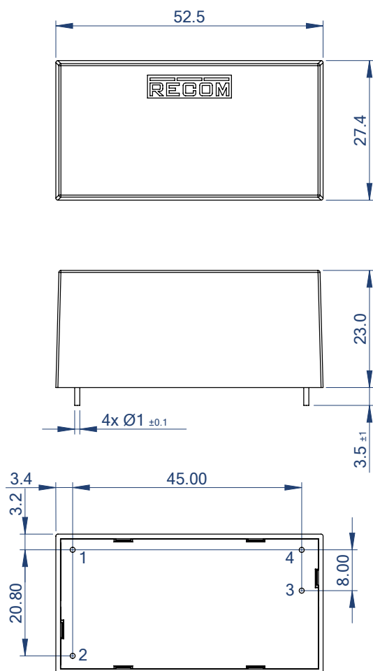
Dimension Drawing (mm)
