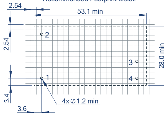
Recommended Footprint Details
