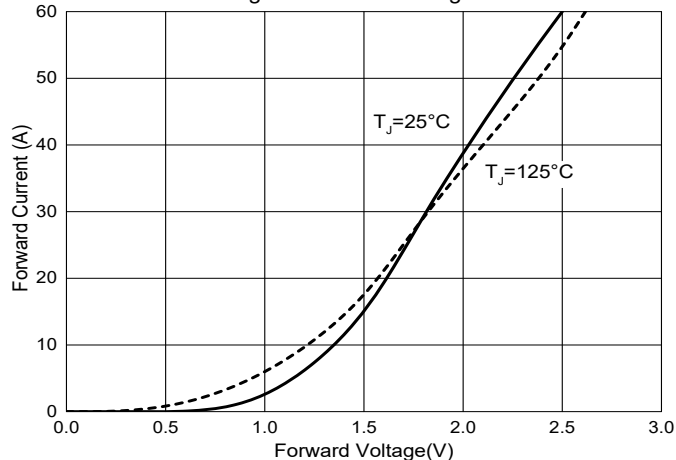
Fig. 6 - Forward Voltage
