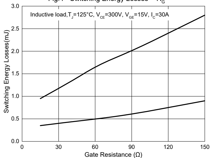
Fig.4 - Switching Energy Losses — R_G
