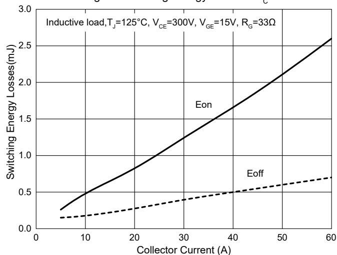
Fig.3 - Switching Energy Losses — I_C
