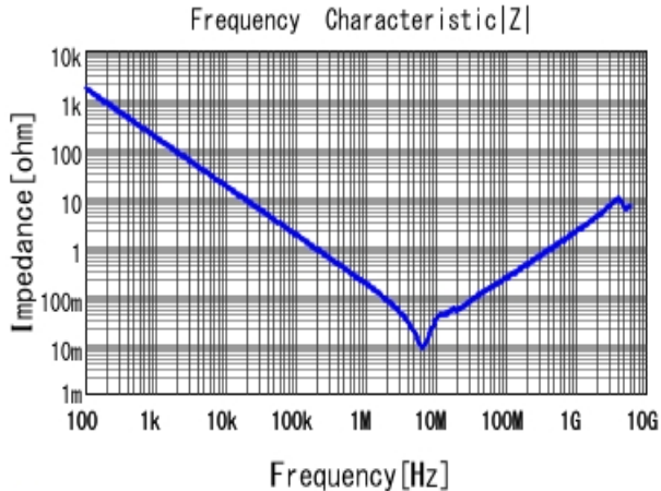
■ GCM21BC72A105ME36 |Z| DC0V, 25degC
