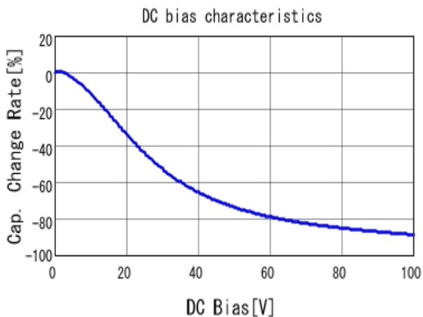
■ GCM21BC72A105ME36 C-DC bias capchange, 25.0degC, AC1.
