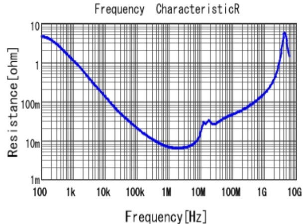
■ GCM21BC72A105ME36 R DC0V, 25degC
