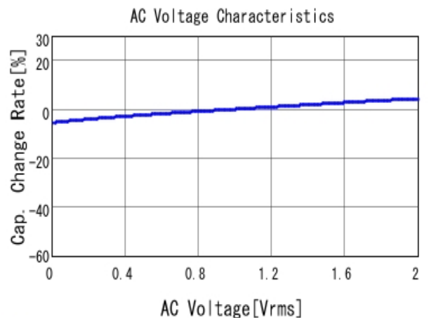
■ GCM21BC72A105ME36 C-AC Voltage capchange, DC0V, 25.0d
