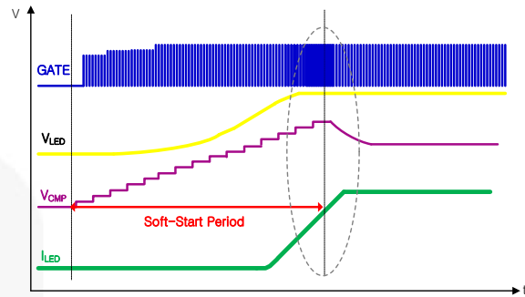
Figure 26. Soft-Start Waveforms
