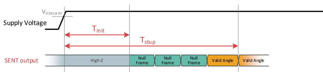
Figure 3 - Startup time definition
