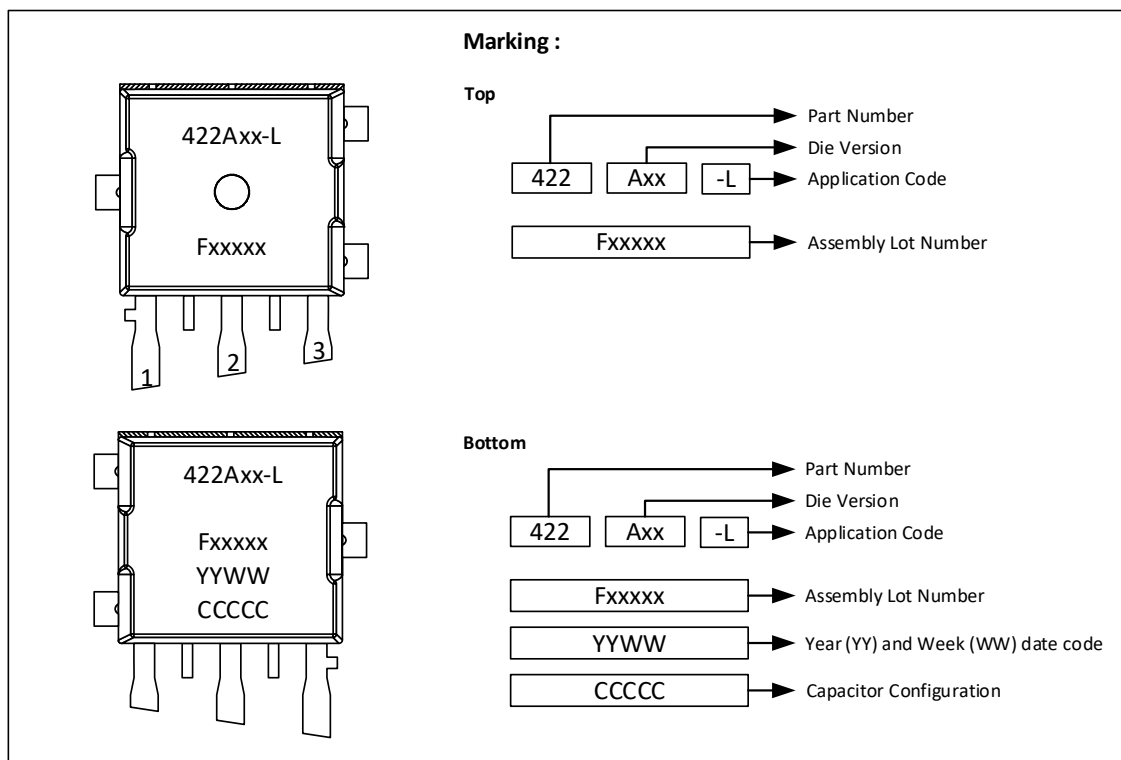
Figure 37 - SMP-3 marking
