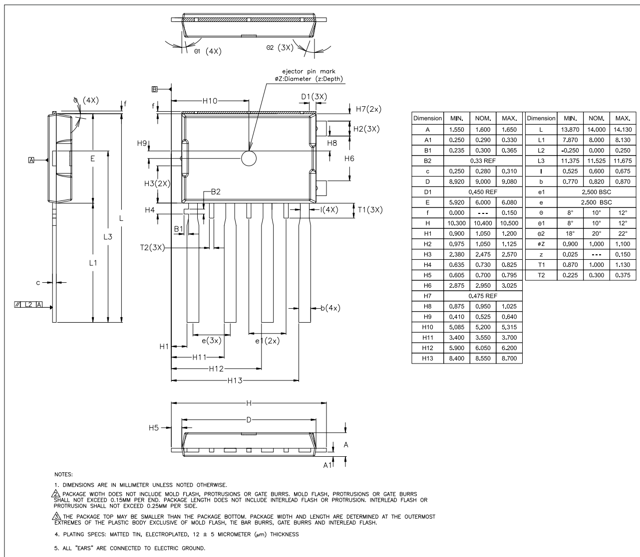
Figure 40 - SMP-4 package outline drawing
