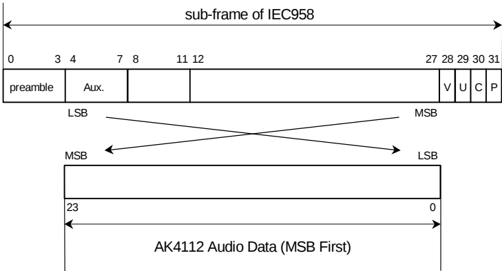
Figure 29. Bit configuration
