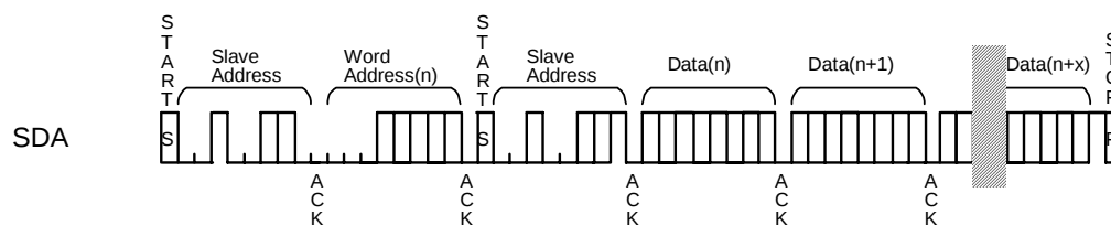
Figure 43. RANDOM READ
