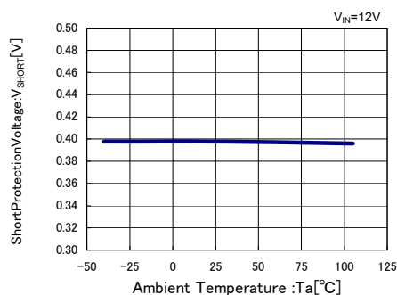
(16) Short Protection Threshold Voltage vs. Temperature
