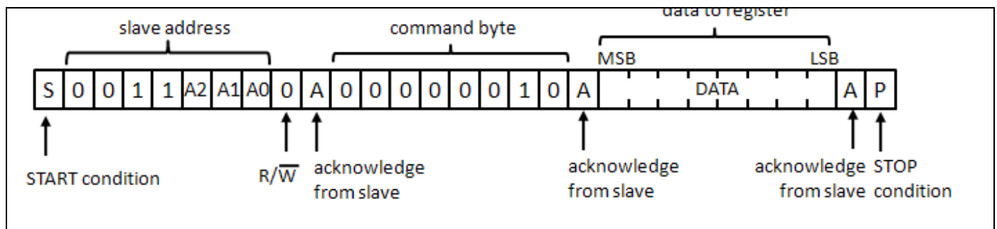
Figure 5. Write to I/O Configuration or Polarity Inversion Registers
