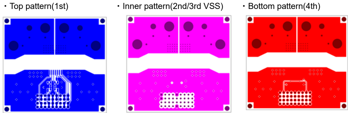
Figure 8. Board layout for measuring thermal resistance of CZ-3A02
