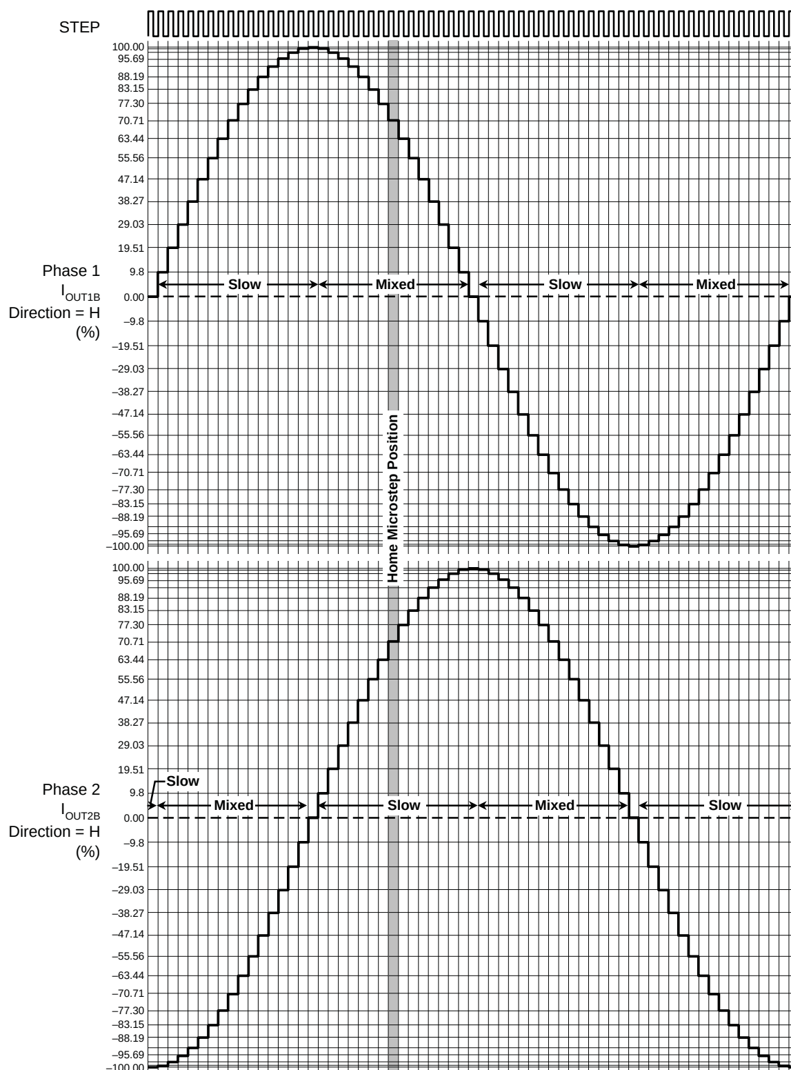
Figure 8. Sixteenth Steps
