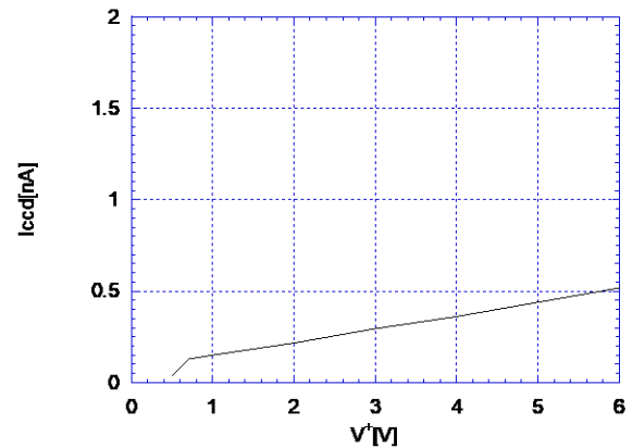
Standby Current vs. Operating Voltage ( V_{CD}=GND , T_a=25^\circ\text{C} )
